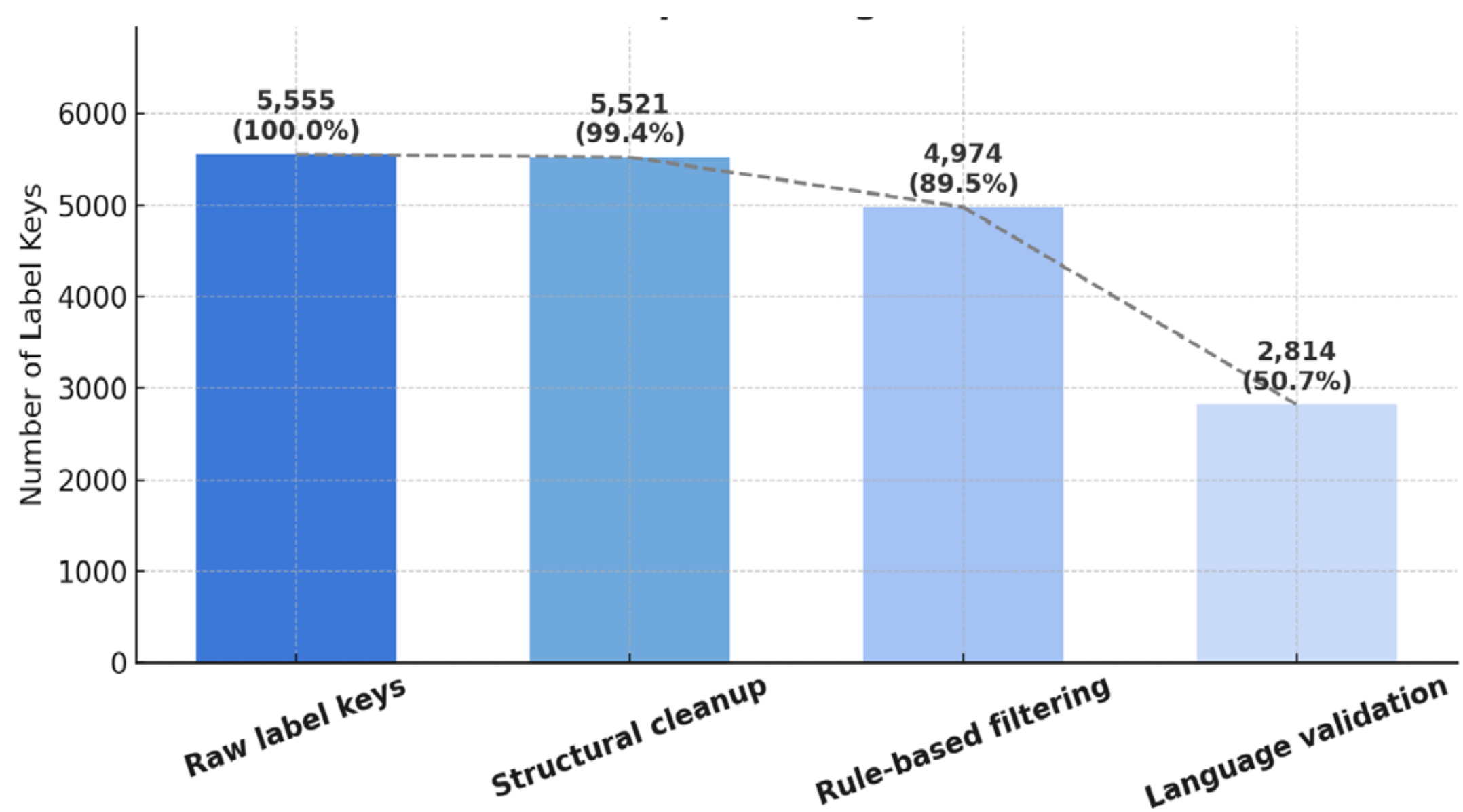
B. Sample-Level Metadata Multi-Step Cleaning Breakdown
